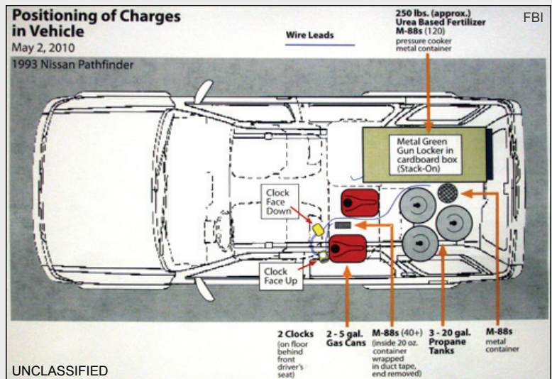
(U) Schematic of vehicle used by Times Square bomber
